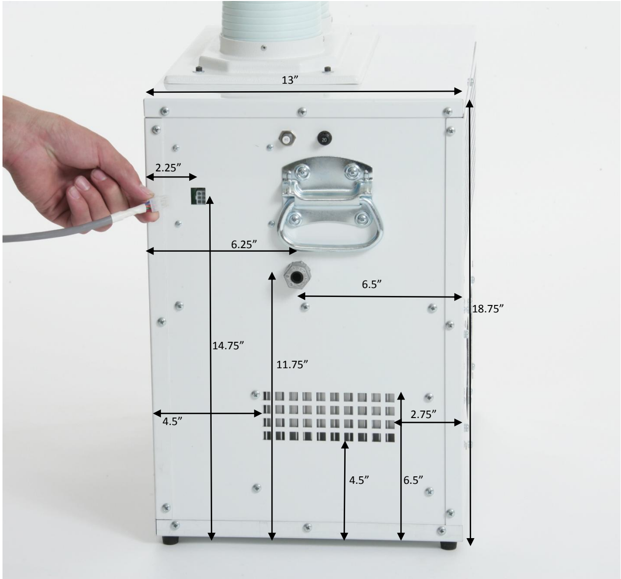
1 RAC 400 Right Side with Dimensions
